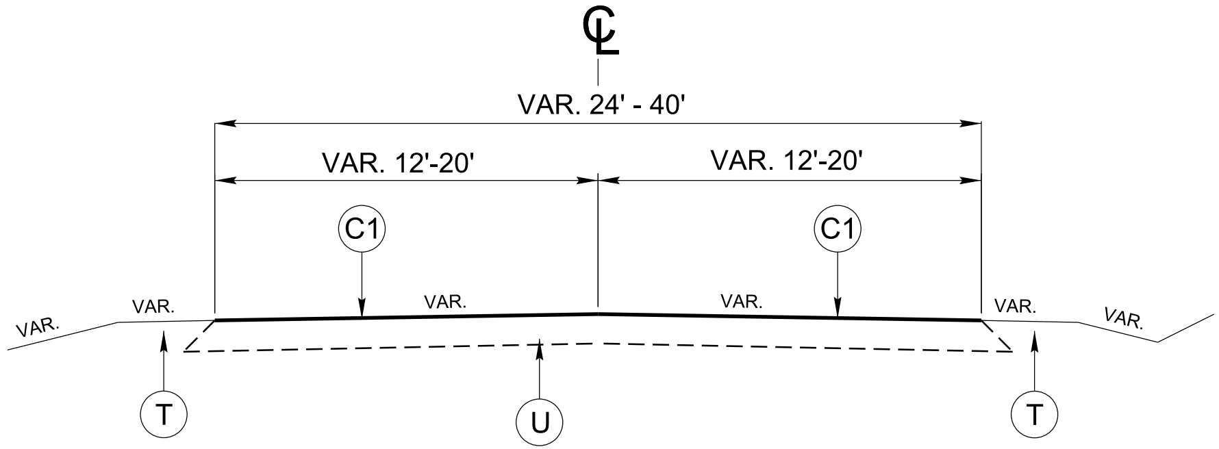
TYPICAL SECTION NO. 1 MAP 1 - US 21 N FROM SURRY CO LINE TO SR 1900
